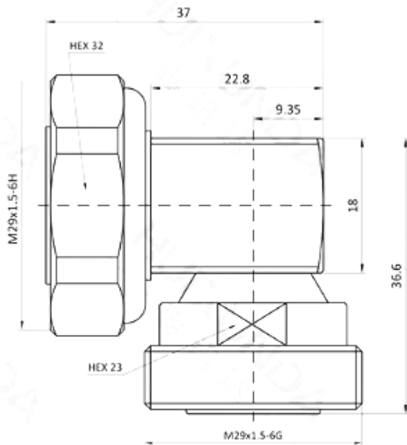
L29 7/16 DIN Male To Female Right Angle Adaptor
