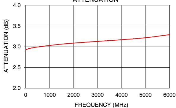
UNAT-3A+ ATTENUATION
