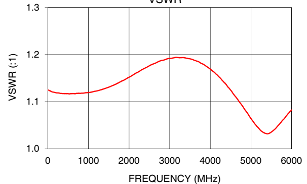
UNAT-3A+ VSWR
