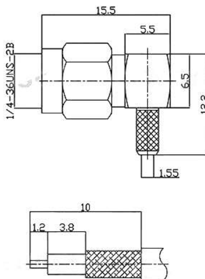
推荐剥线尺寸 Recommended stripping size
