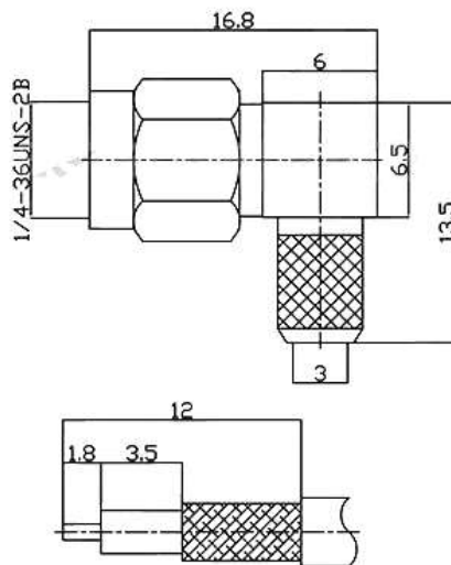
推荐剥线尺寸 Recommended stripping size
