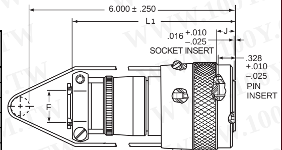
Breakaway PT-CE with Crimp Contacts, Environmental with Strain Relief 71-3395XX-( ) 72-3395XX-( )
