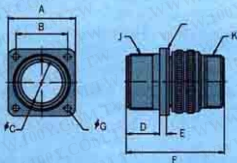
MS 3100 壁式安裝插座 Wall Mounting Receptacle
