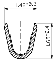
SECT. X-X
