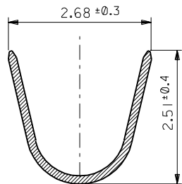
SECT. Y-Y
