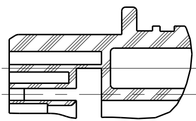
SECTION F-F
