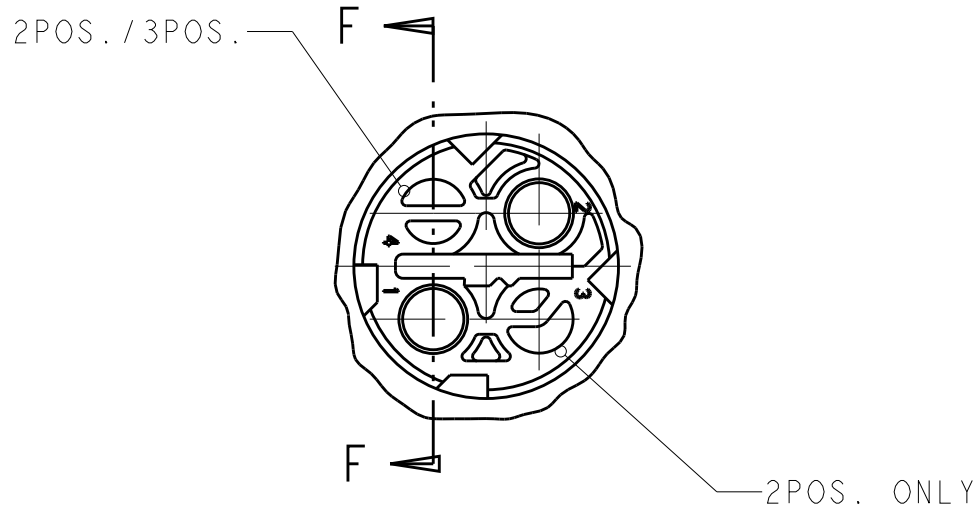
CLOSED CAVITY OF THE 2POS./3POS. SOCKET HOUSING
