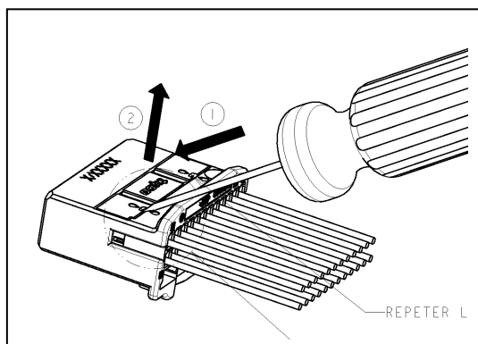
Fig.20 Ouverture du verrou Opening of retainer
