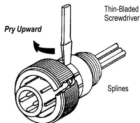
Removing Damaged Coupling Ring
