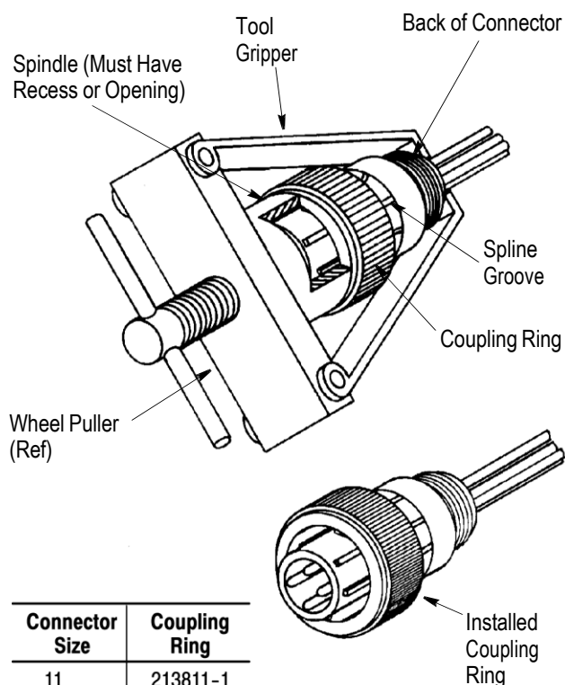
Installing Coupling Ring
