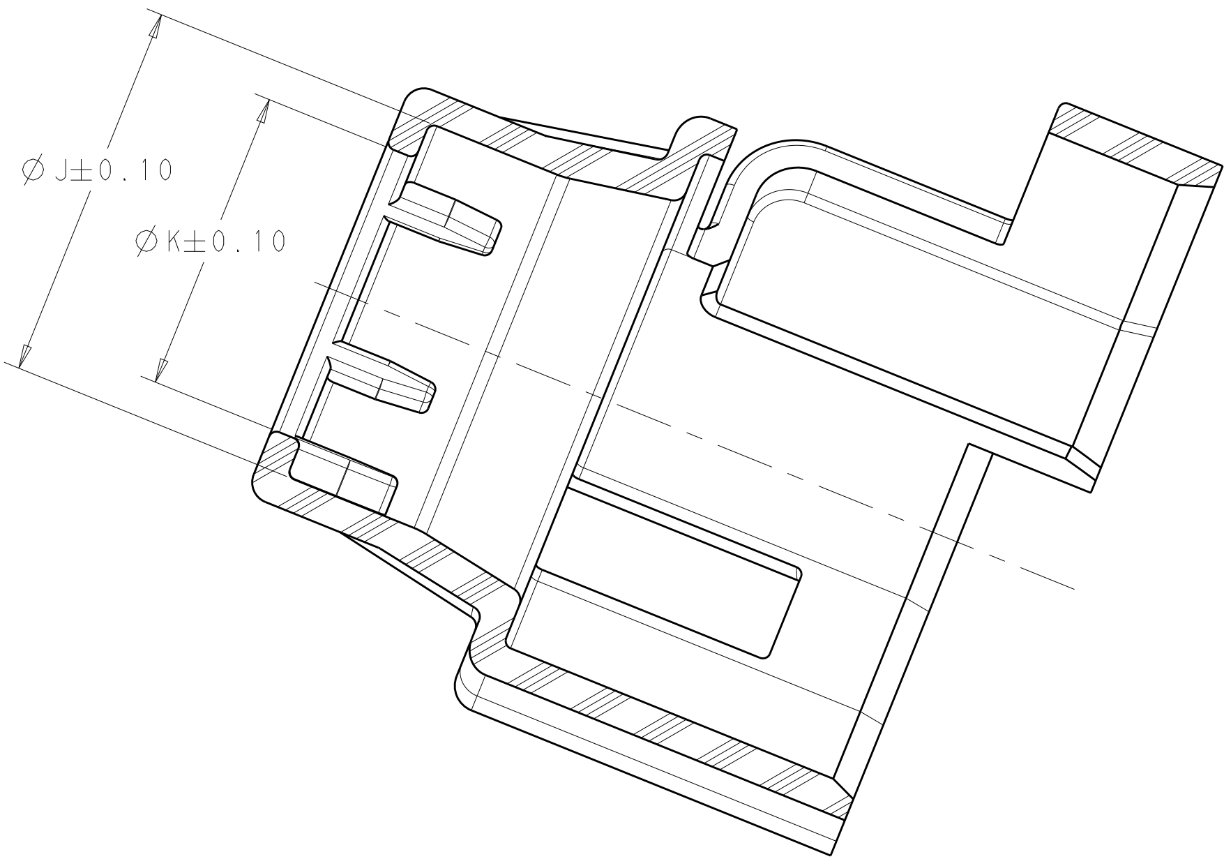
SECTION C-C
