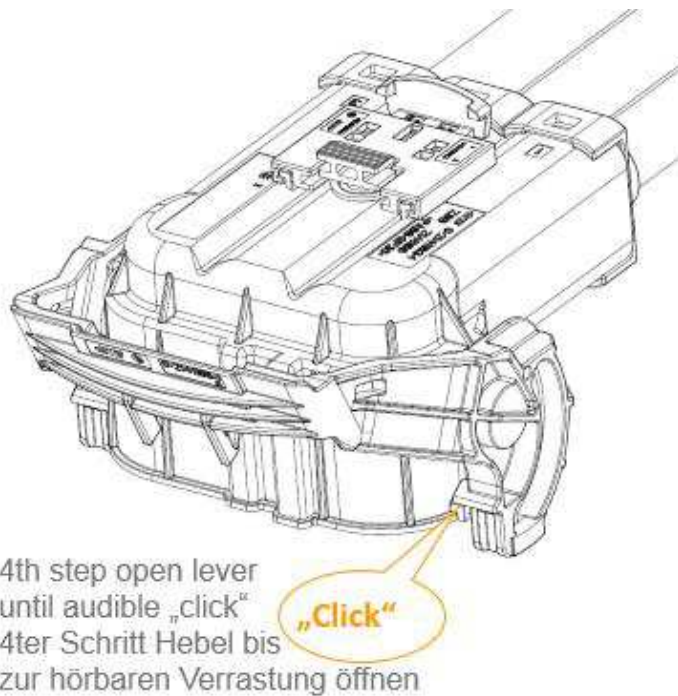
Figure 22: Plug position of lever
