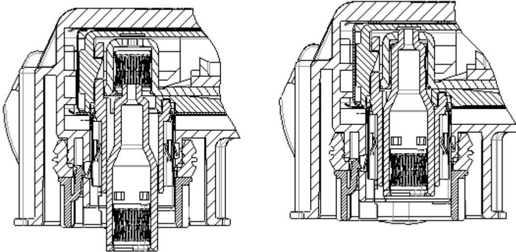
Figure 16: Insert contact pin
