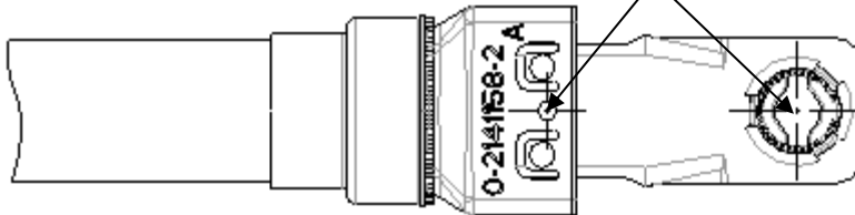
Figure 9: Shield crimp Abbildung 9: Schirmcrimp
