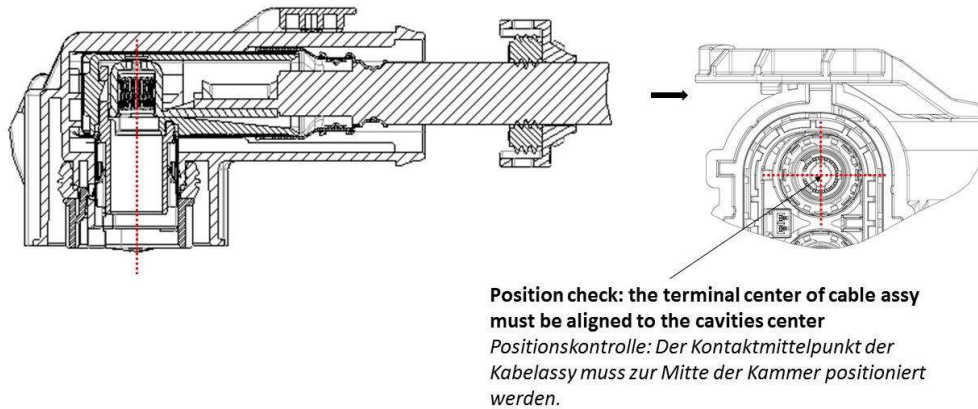
Figure 14: INSERT CABLE ASSEMBLY INTO THE RECEPTACLE HOUSING
