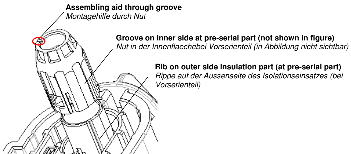
Figure 17: Finger protection cap aligned to insulation part.
