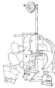
AMP-O-ELECTRIC Model "K" Terminator Machines 565435-5 or 1-471273-2 (409-5128)
