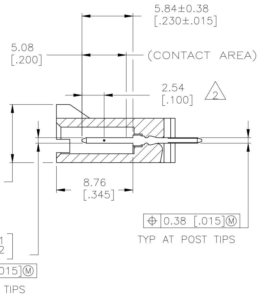
SECTION X-X
