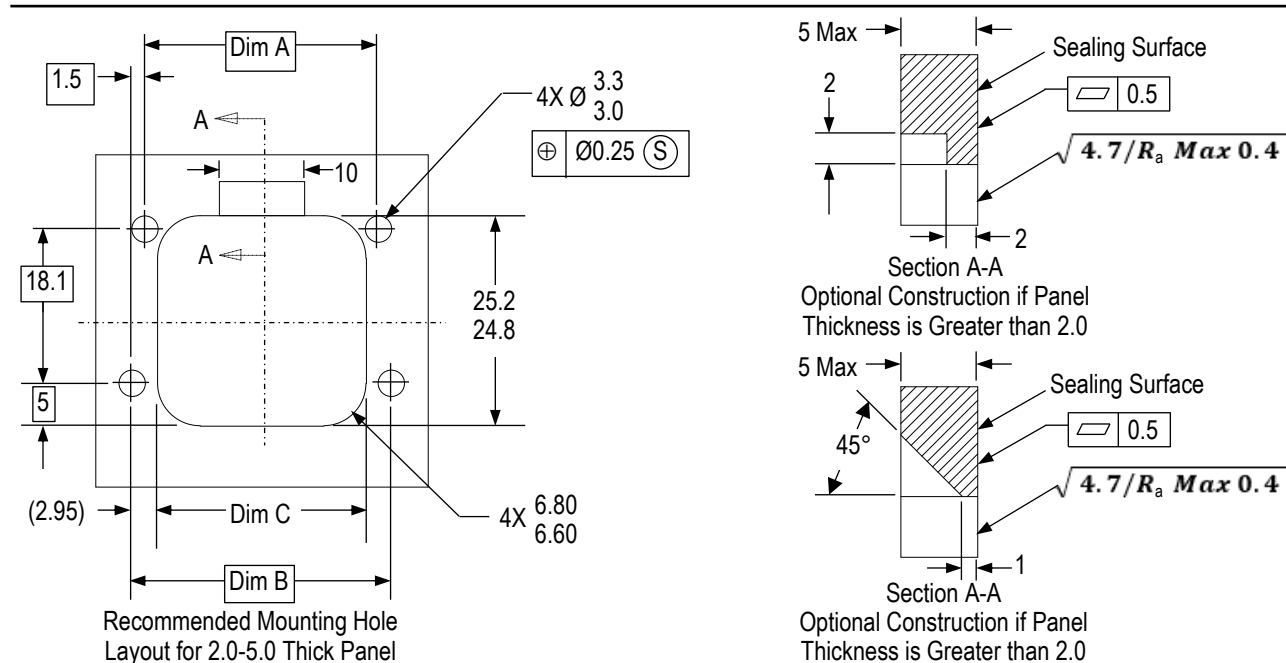
PANEL CUTOUT DIMENSIONS
