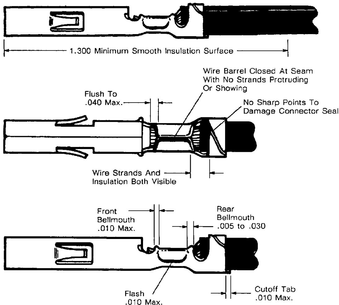
Fig. 2. Crimping Requirements (cont'd)
