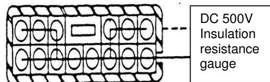
<Figure 3-7:Between neighboring terminal and housing surface>
