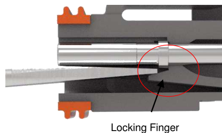
Locking Finger
