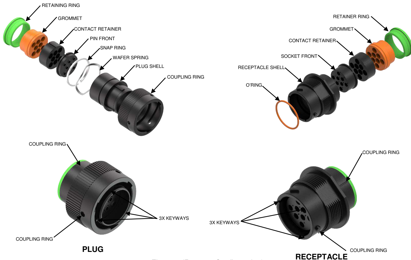
Figure 2 (Reverse Configuration)
