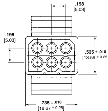
Plug
