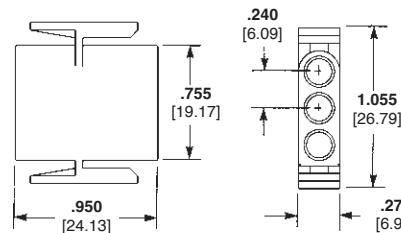
Socket Housing (Plug)
