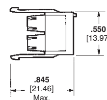
Cap Rear
