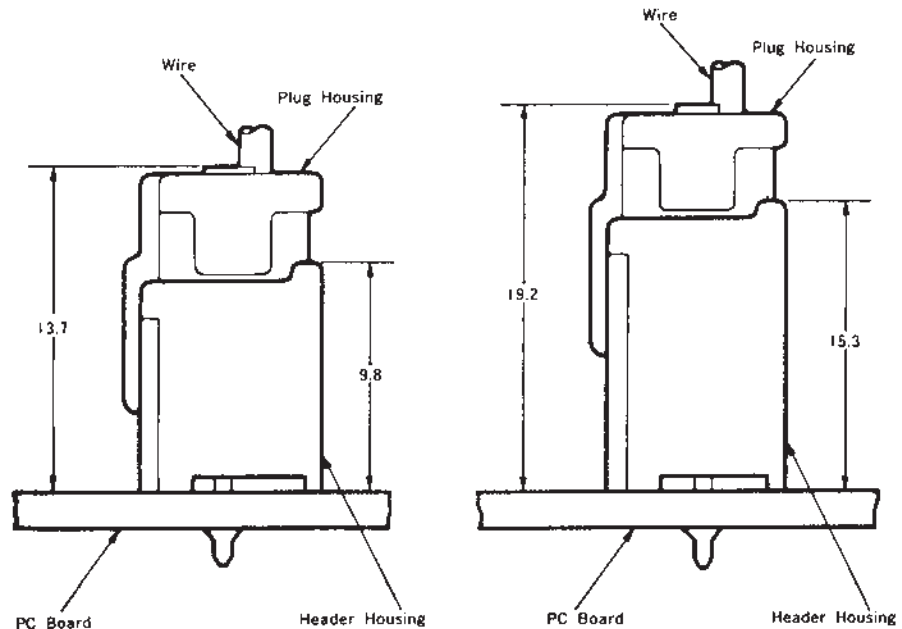
Standard-Profile Type
