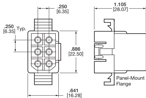
Plug
