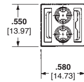
Plug Rear
