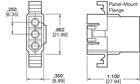
Plug
