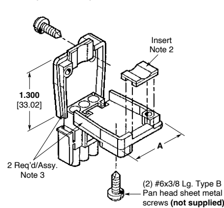
In-Line
