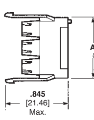
Cap Rear
