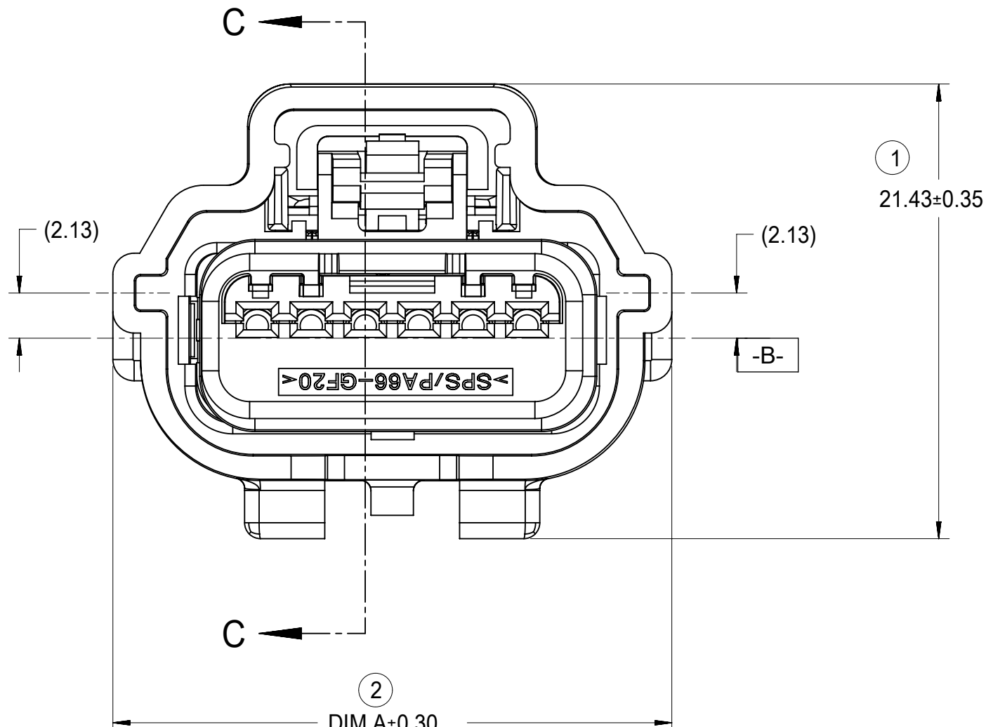
FRONT VIEW
