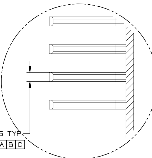
DETAIL N SCALE 5:1
