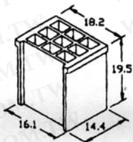
JP1731-9K MATERIAL : NYLON
