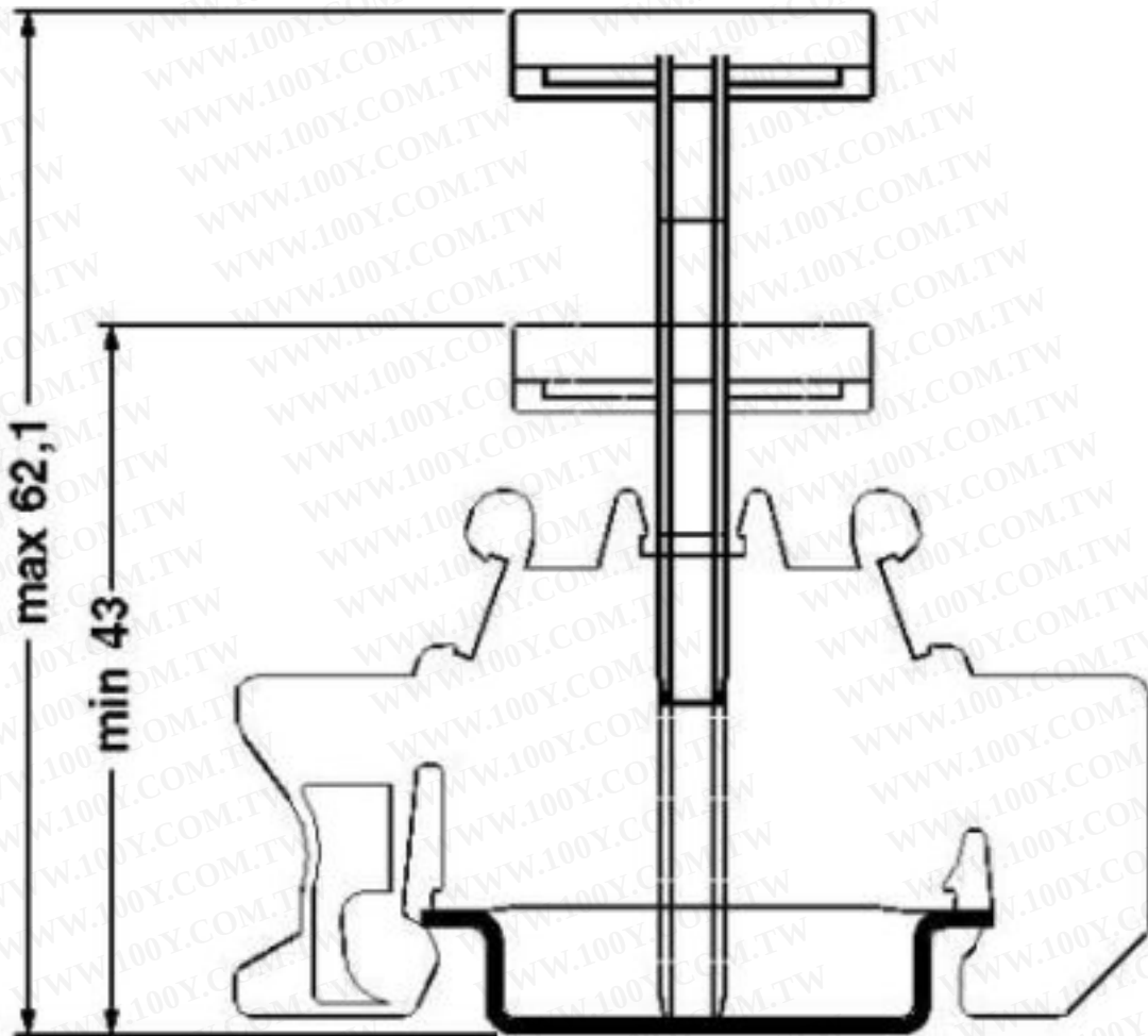
Dimensional drawing
