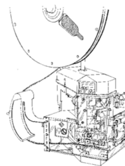
AMP-O-ELECTRIC Model "G" Terminating Machine 354500-[] (409-5842)
