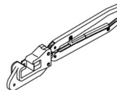
Hand Crimping Tool 69710-1 (408-2095)
