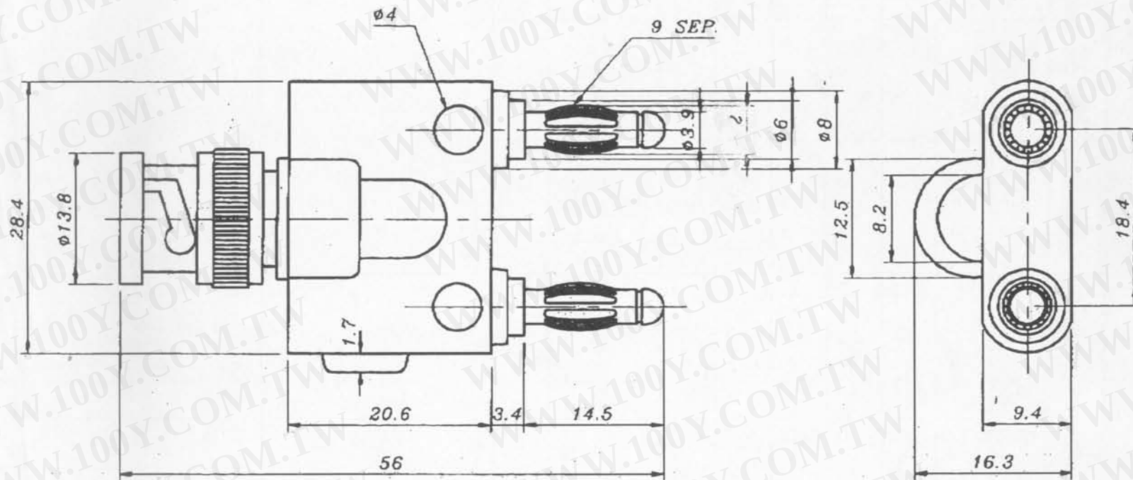
BNC PLUG TO DUAL BANANA PLUG
