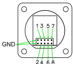
PIN ASSIGNMENT REAR VIEW(後視圖)
