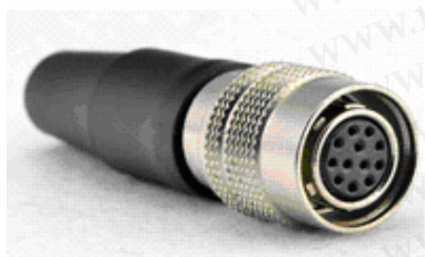
HR10A-10P-12S
