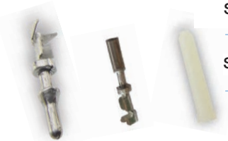
Pin Socket Wire hole filler *
