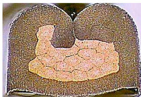
Uneven Crimp and Wall Thickness and Flash on Both Sides
