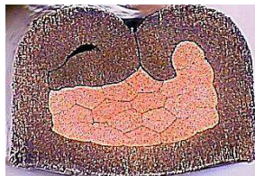
Uneven Crimp and Wall Thickness
