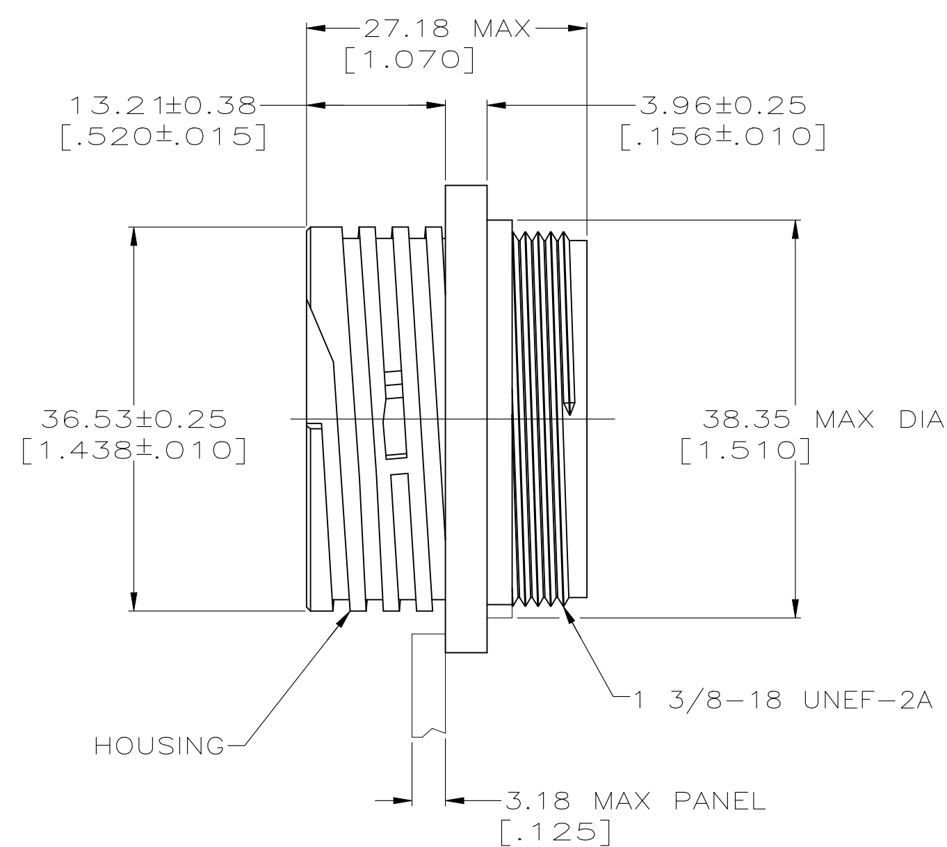
DETAIL A
