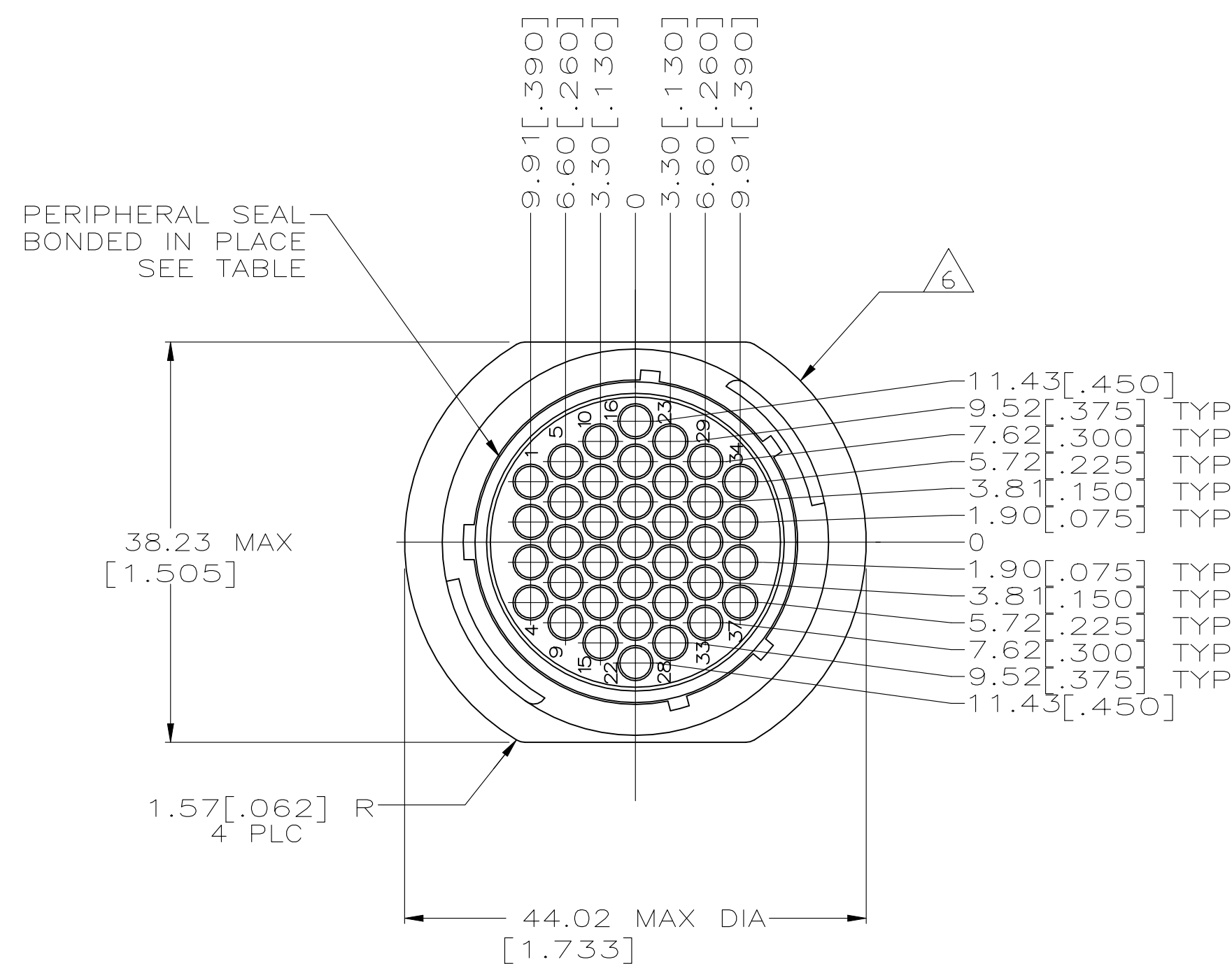
DETAIL B
