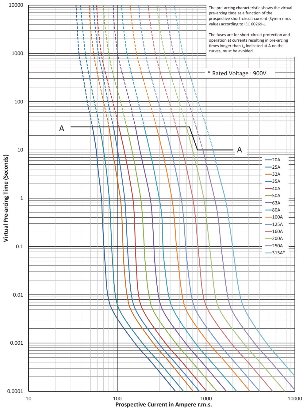
Time-current curve - 20 A to 315 A
