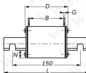
With blown fuse indicator
