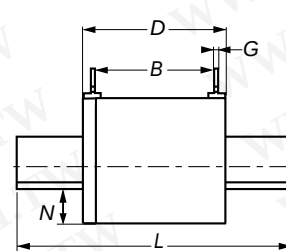
With blown fuse indicator
