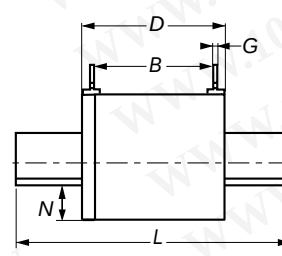
With blown fuse indicator
