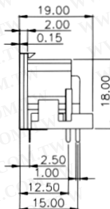
Dimension (m/m)
