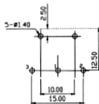
P.C.B Layout Jack Bottom View
