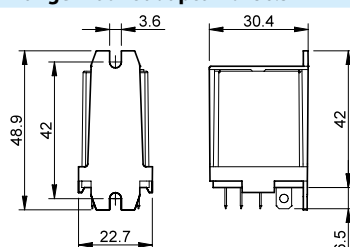
056.26 with relay
