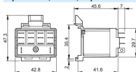
056.47 with relay
