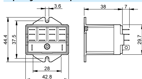
056.45 with relay
