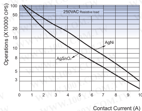
ENDURANCE CURVE
