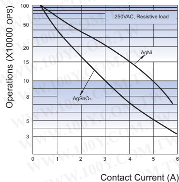
ENDURANCE CURVE
