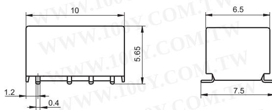
Standard SMT type
