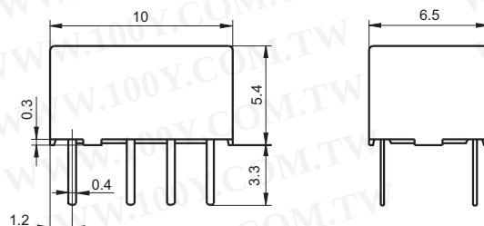
Outline Dimensions
