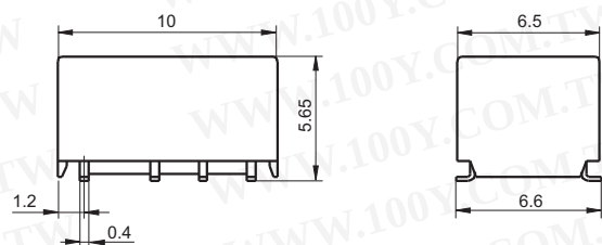
Short terminal SMT type
