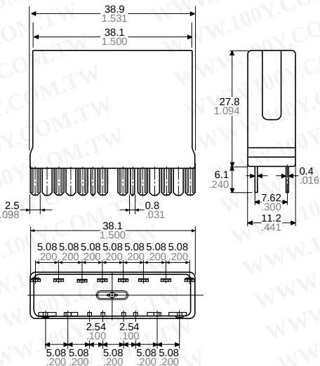
External dimensions
