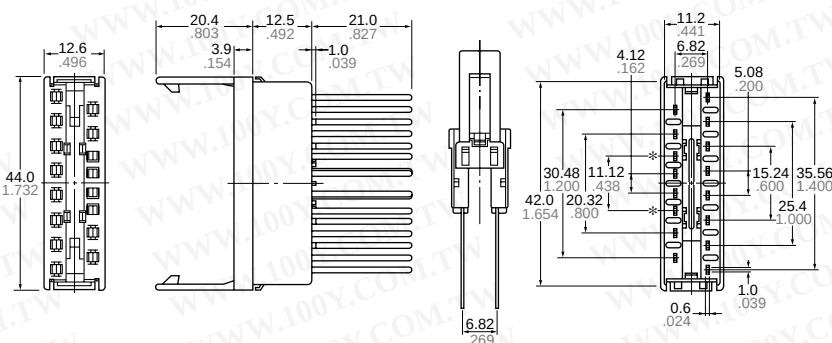
External dimensions
