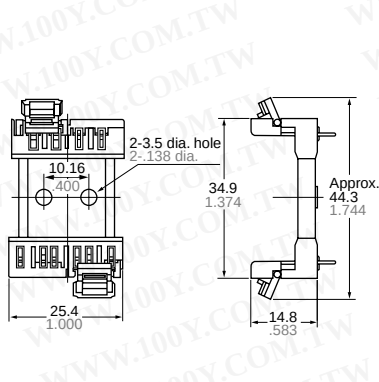
External dimensions
