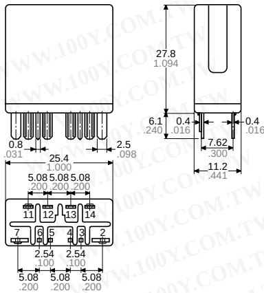
External dimensions
