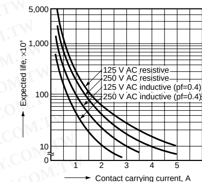
1.-(3) Life curve (AC/DC load 4 Form C)
