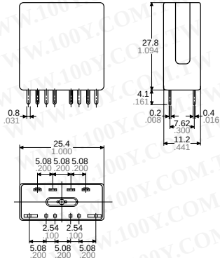
External dimensions
