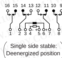
Schematic (Top view)
