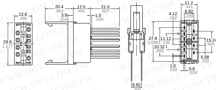
External dimensions
