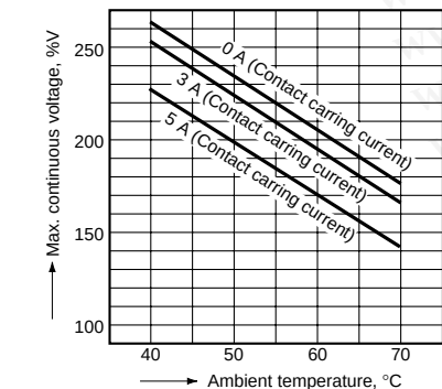
6.-(1) Ambient temperature vs Max. continuous voltage Tested sample: NC2D-P-DC24 V (2 Form C slim single side stable)
