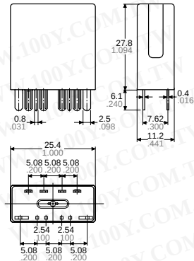
External dimensions
