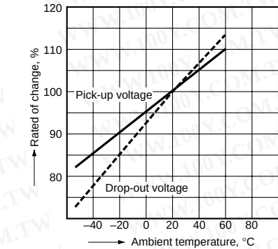
5.-(2) Rate of change of pick-up and drop-out voltage (4 Form C single side stable)
