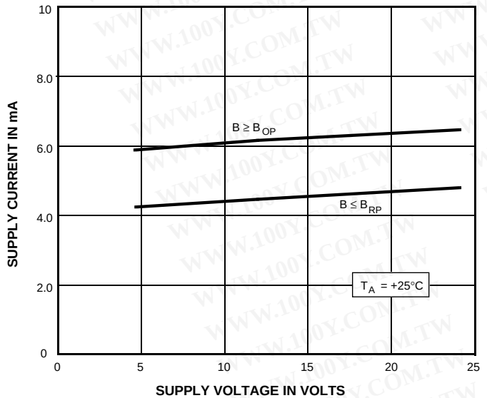
SUPPLY CURRENT
