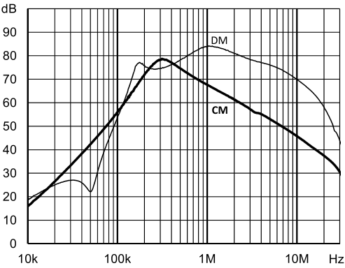
FN3288-63-53-C35-R65
