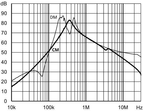
FN3288-125-35-C35-R65
