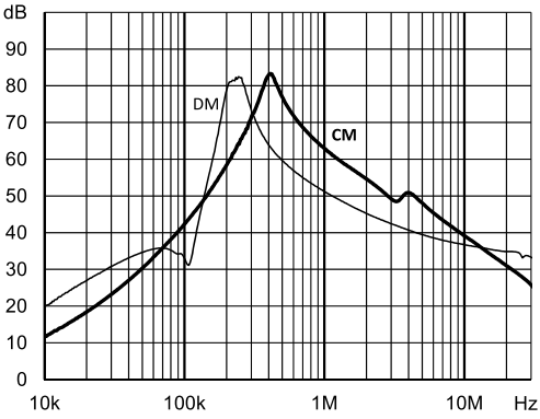
FN3287-160-40-C33-R65
