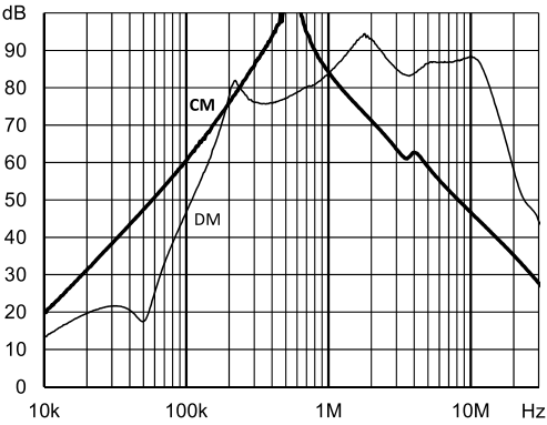
FN3288-25-33-C35-R65
