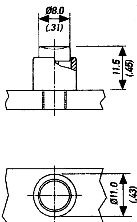
Round Button PBR Round Bezel BZR
