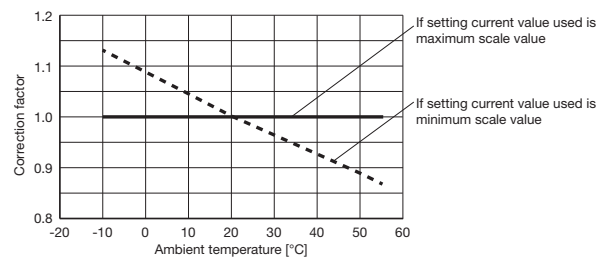
Fig. 6-1 TR18X, TR38X
