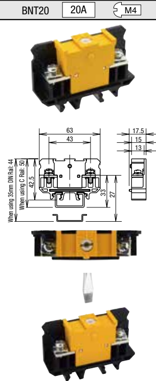
Self-Lifting Terminal with Disconnecting Switch
