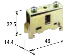
BNL8 (M4 Screw) (*3)
