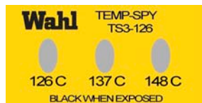
Economy Three-Position Base Part No. TS3 .75" X 1.5" (19 X 38mm) Shipped in bags of 20
