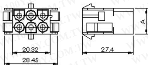
6 Circuit (Matrix)
