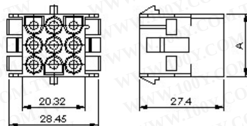
9, 12, 15 Circuit (Matrix)
