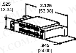
Mating Face
