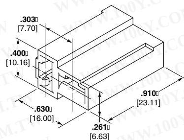
Receptacle Housing
