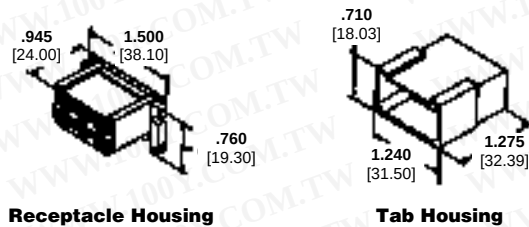
Receptacle Housing
