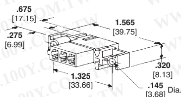
Receptacle Housing
