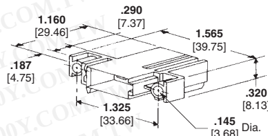
Tab Housing
