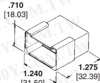
Tab Housing
