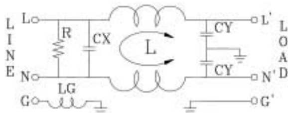
ELECTRICAL SCHEMATIC 3
