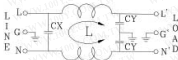
ELECTRICAL SCHEMATIC 1
