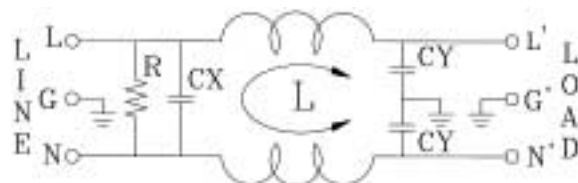
ELECTRICAL SCHEMATIC 2
