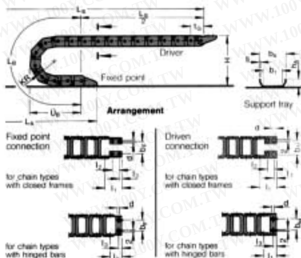
Chain type 0450.61 with hinged bows
