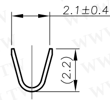
Sec. B-B
